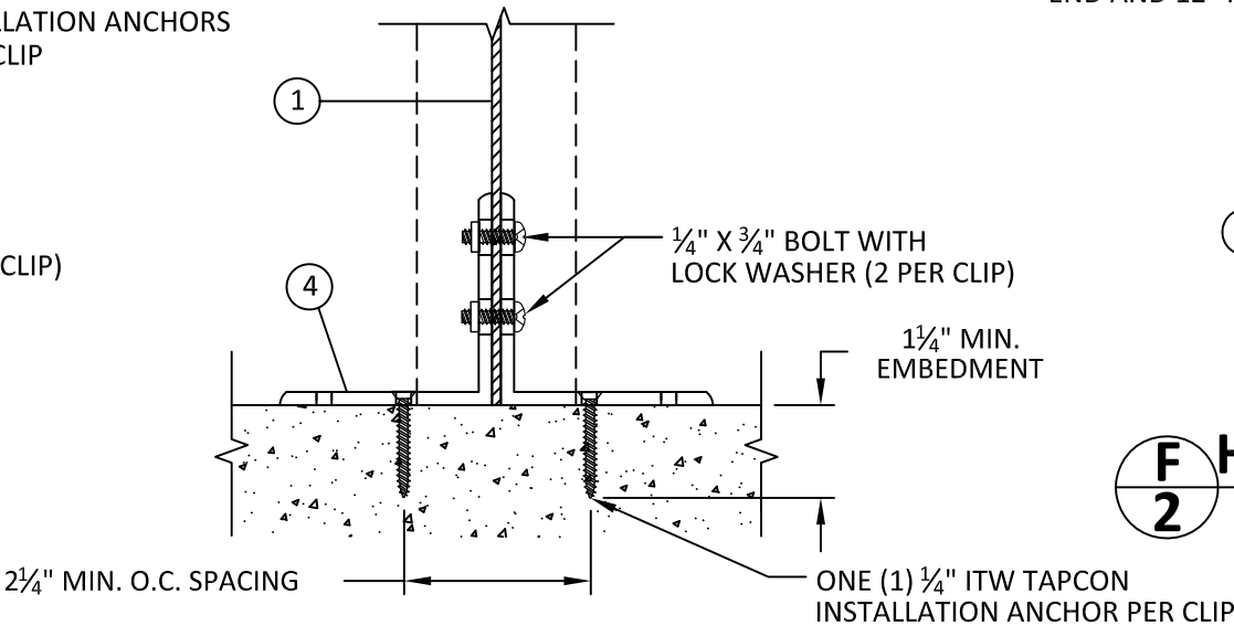
C 2 FRONT VIEW SILL - CONCRETE/MASONRY MULLION CLIP
