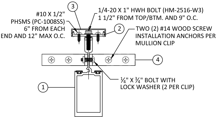
F 2 HORIZONTAL SECTION 2X WOOD MULLION CLIP
