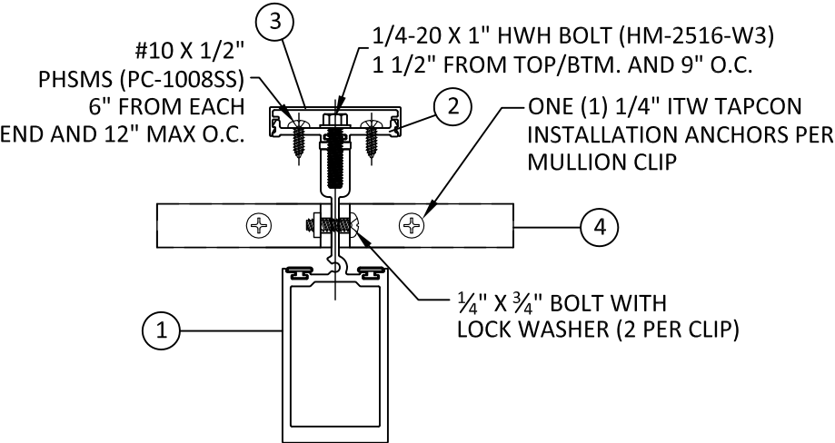
D 2 HORIZONTAL SECTION CONCRETE/MASONRY MULLION CLIP
