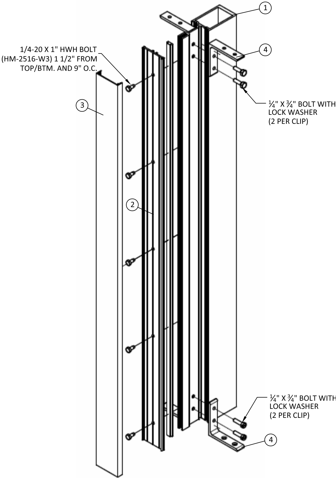
4562 STACKING MULLION ASSEMBLY TYPICAL
